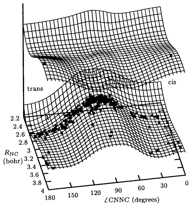
Figure 2. Photolysis of the isolated molecule, TSH simulation. \Delta CNNC and R_{NC} coordinates for each trajectory at the time of the first surface hopping. The two PES are represented schematically (no geometry optimization) and the S_1 PES is shifted upward for a better view of the lower one.
