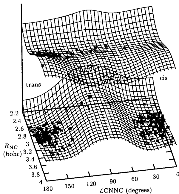
Figure 3. Photolysis of the isolated molecule, TSH simulation. \Delta CNNC and R_{NC} coordinates for each trajectory at the time t = 1 ps. Same surfaces as in Figure 2.
